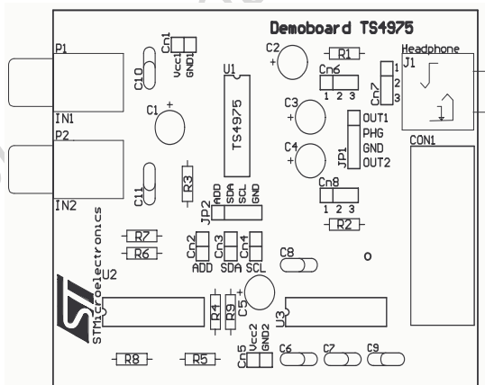
Figure 66. Component location
